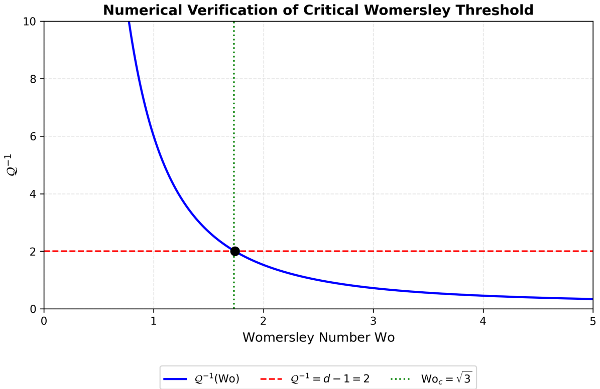
Figure 1: Numerical verification of the critical Womersley number. The inverse quality factor Q^{-1} (blue curve) intersects the geometric constraint Q^{-1} = 2 (red dashed line) at \text{Wo} \approx 1.74 , matching the analytical prediction of \sqrt{3} (green dotted line).
